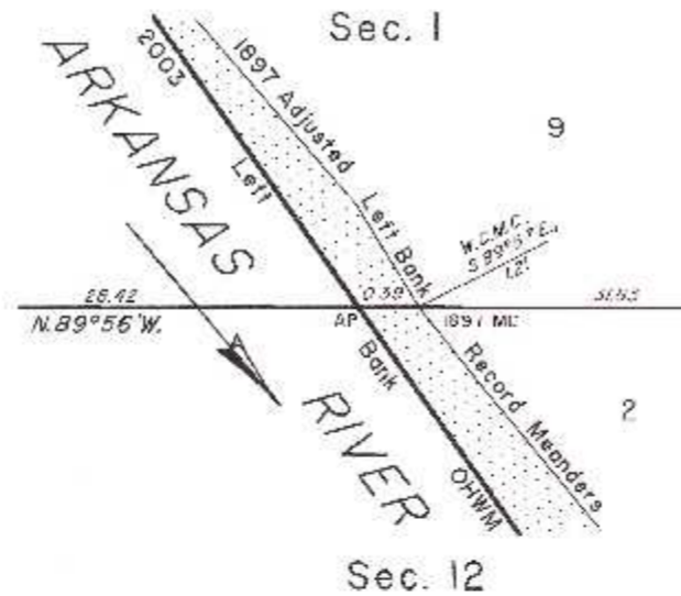
ENLARGED DIAGRAM No. 2 (Not to Scale)
