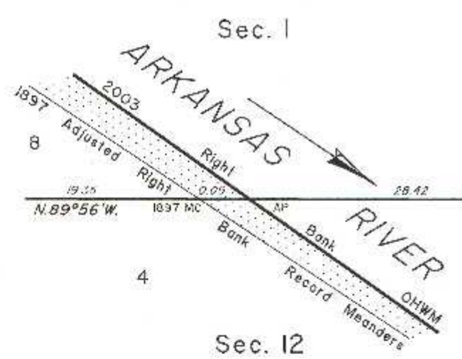
ENLARGED DIAGRAM No. 1 (Not to Scale)
